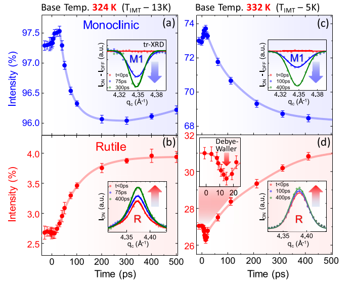
FIG. 7. Structural dynamics of the crystalline \text{VO}_2 (001) thin film undergoing an IMT induced by an ultrafast THz electric-field pulse with 1-MV/cm peak electric field. (a), (b) Long-term temporal evolution of the monoclinic (a) and rutile (b) peak intensities, obtained via \theta - 2\theta scans (shown in the insets) at each time delay at a base temperature of 324 K. (c), (d) Temporal evolution of the monoclinic (c) and rutile (d) peak intensities at a higher base temperature of 332 K. The insets in panels (a)–(d) show the \theta - 2\theta scans at key time delays: before the excitation (red), approximately halfway to the saturation point (blue), and near the saturation point (green). Experimental spectra (circular markers in the insets) were fitted using simple Gaussians (solid lines) to obtain peak intensities as functions of time delays. For the monoclinic peak, since the intensity changes are significantly smaller compared to the absolute intensities of the peak in the ground state ( \sim 73 – 97\% ), we show the angle-resolved intensity change spectra ( I_{\text{ON}} - I_{\text{OFF}} ). These were obtained by subtracting the reference \theta - 2\theta scans recorded without the excitation laser pulse ( I_{\text{OFF}} ) from the normal scans obtained with the laser pulse ( I_{\text{ON}} ). Upper inset in panel (d) shows the initial suppression of the rutile x-ray diffraction signal [absent in (b)] for the first 15 ps due to preferential heating of the lattice in these metallic regions.
