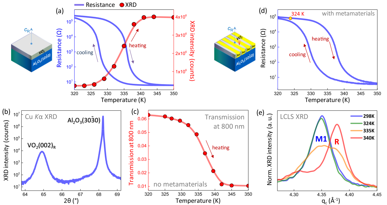
FIG. 1. Static resistance and x-ray diffraction characterization of the 200-nm \text{VO}_2(001) film deposited on \text{Al}_2\text{O}_3(10\bar{1}0) substrate. (a) Resistance versus temperature curves (blue) showing the insulator-metal transition during both heating and cooling cycles for the unpatterned film. Also shown is the intensity of the \text{VO}_2(002)_R diffraction peak measured with synchrotron radiation and plotted as a function of temperature. (b) High-resolution \text{Cu } K\alpha \theta - 2\theta x-ray diffraction pattern showing both the substrate and the film Bragg peaks. (c) Static near-IR (800-nm) transmission versus temperature measured on the unpatterned film during the heating cycle. Temperature scale was adjusted to account for the difference in the temperature calibration between the different sample holders. (d) Resistance versus temperature curves measured after patterning the \text{VO}_2 film with Au metamaterials. Starting (base) temperature for the pump-probe measurements (324 K) is marked with a yellow circle. (e) Temperature-dependent x-ray diffraction scans of the \text{VO}_2 film peak carried out at LCLS prior to time-resolved measurements.
