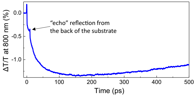
FIG. 6. THz-pump-near-IR-probe change in transmission for \text{VO}_2/\text{Al}_2\text{O}_3 for longer time delays. Transmission at 800 nm decays monotonically, with the exception of a sharp feature observed at ca. +9.5 ps time delay, which is an echo artifact, arising due to the reflection of the THz pulse from the backside of the substrate in the normal-incidence geometry.
