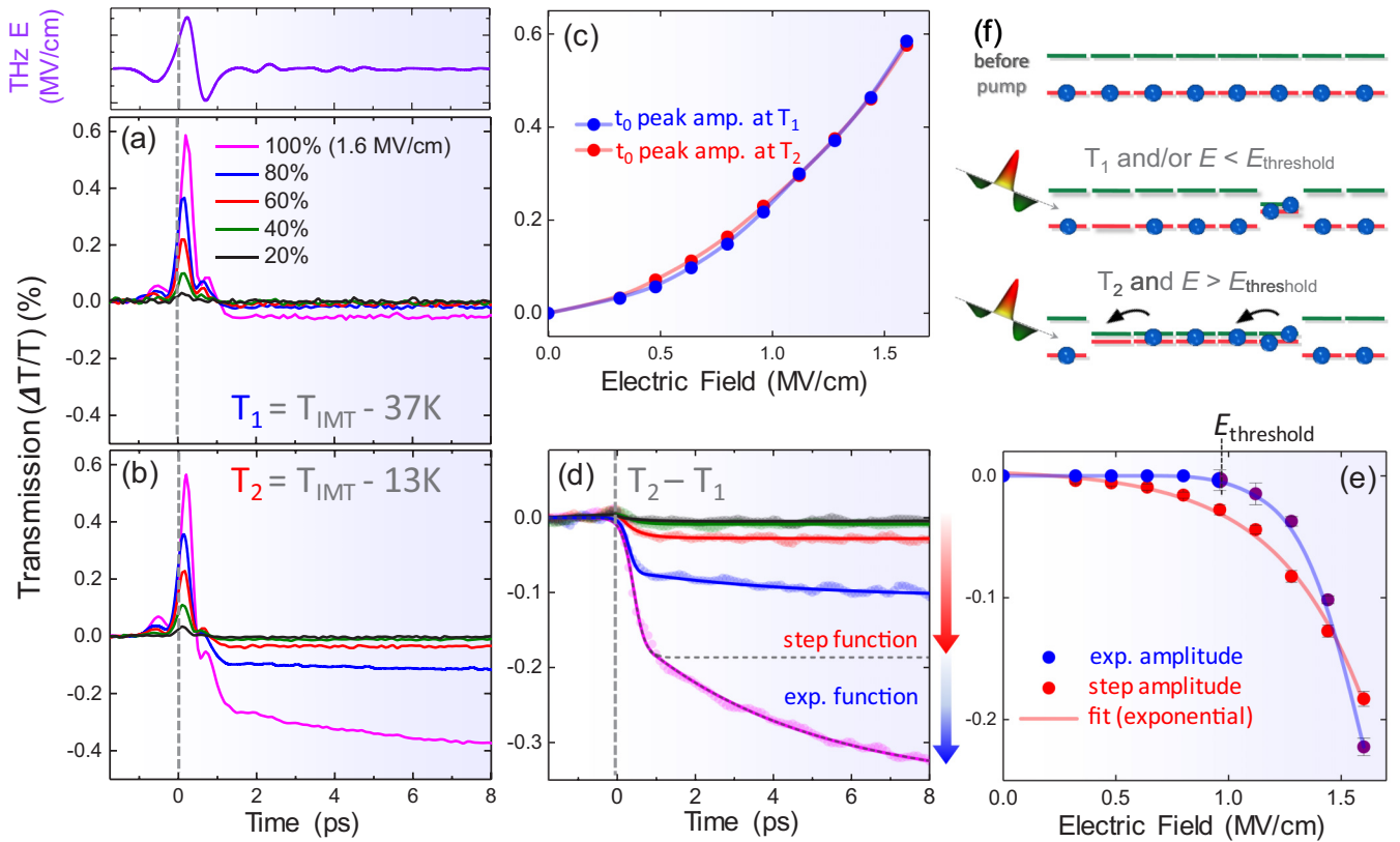
FIG. 5. Electronic dynamics in a VO 2 thin film undergoing an IMT induced by an ultrafast THz electric-field pulse [shown in the outset above panel (a)]. (a) The E -field-dependent electronic response measured via near-IR transmission at room temperature ( T_1 = 300 K) is dominated by a sharp transient increase in transmission consistent with Wannier-Stark-like band renormalization [3,33–38]. For high fluences (e.g., purple delay trace) this process is accompanied by a weak concomitant drop in transmission, characteristic of sudden metallization of VO 2 via direct Zener-Keldysh-like interband tunneling [38–42]. (b) At the onset of the IMT ( T_2 = T_{\text{IMT}} - 13 K) tunneling processes become more efficient, and above a threshold peak field of approximately 1 MV/cm the absorbed energy density is sufficient to initiate lattice dynamics (see Fig. 7). (c) Wannier-Stark peak amplitude exhibits a nonlinear dependence on the peak E field with minimal temperature dependence between 300 and 324 K. (d) The subsequent dynamics can be pictured more clearly by subtracting off the temperature-independent dynamics. In this plot, data shown in panel (a) are subtracted from the corresponding data from panel (b). (e) E -field dependence of the amplitudes characterizing the pulse-width-broadened step and exponential functions suggests different electronic origins of the two processes and reveals the threshold onset of the exponential feature. (f) Schematic representation of the early-time electronic dynamics. The scenarios discussed in the text are visualized by depicting schematic energy levels (metallic vs insulating) for an atomic chain.
