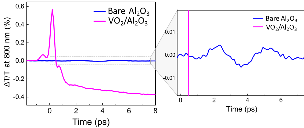
FIG. 4. Substrate response to the THz E -field pump. THz-pump–near-IR-probe change in transmission response for the bare \text{Al}_2\text{O}_3 substrate (blue) compared to that of a 200-nm \text{VO}_2 film on the same \text{Al}_2\text{O}_3 substrate (magenta). The \text{Al}_2\text{O}_3 substrate shows almost no measurable response to the THz pulse, except for small-amplitude ps-scale modulations between 2 and 6 ps (outset) which are orders of magnitude weaker than the \text{VO}_2 response.
